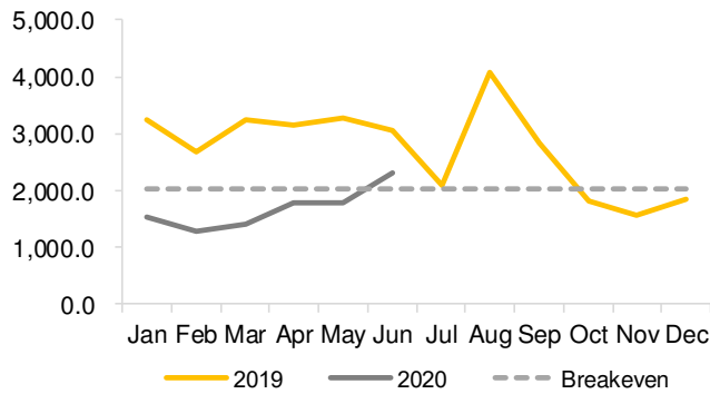
Figure 1: Water flow at XPCL (CMS)
