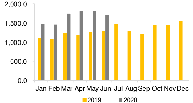
Figure 6: Electricity generation at BKC (MWh)
