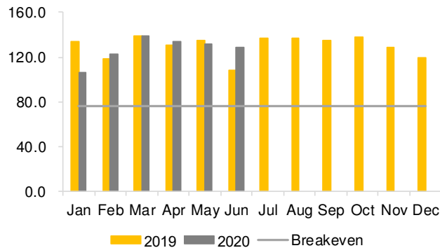
Figure 5: Electricity generation at BIC (GWh)
