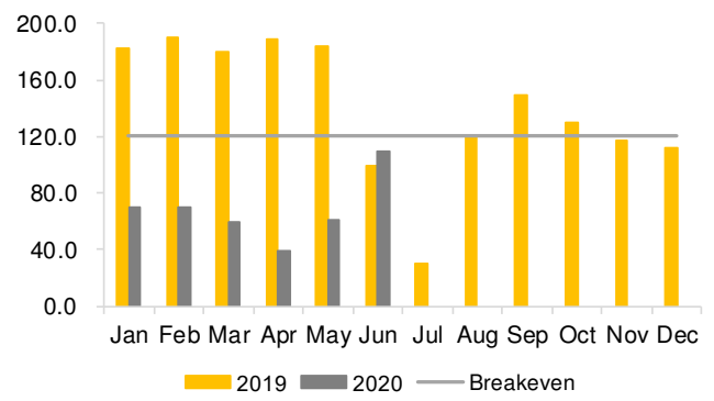
Figure 4: Electricity generation at NN2 (GWh)
